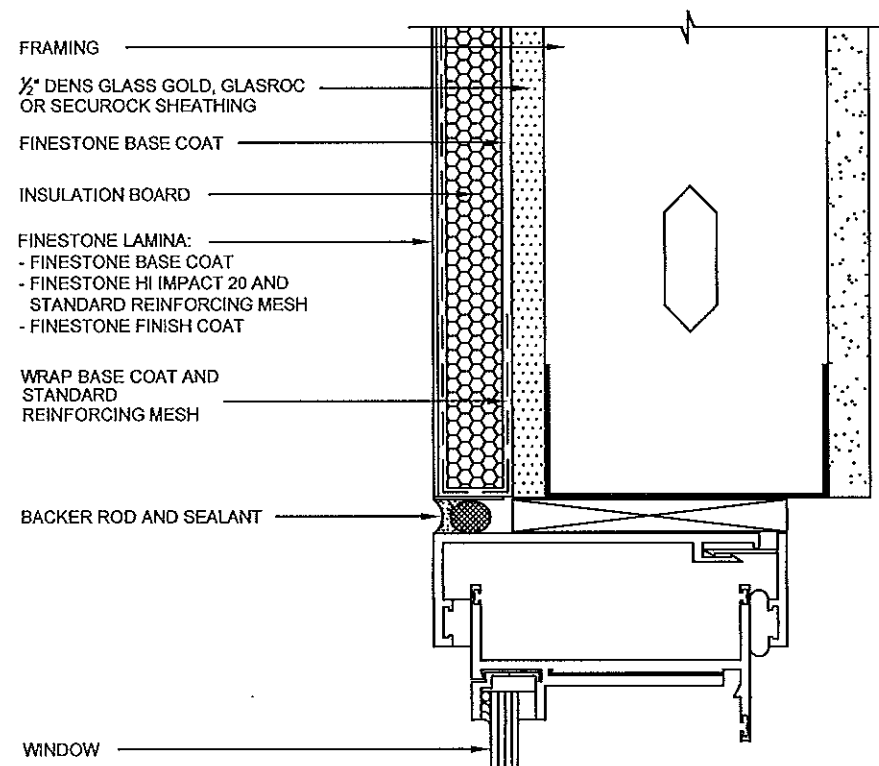
WINDOW HEAD (FLUSH)
