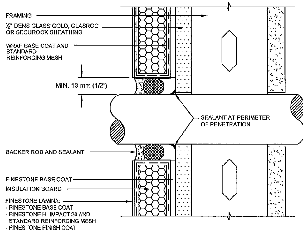
PIPE PENETRATION
