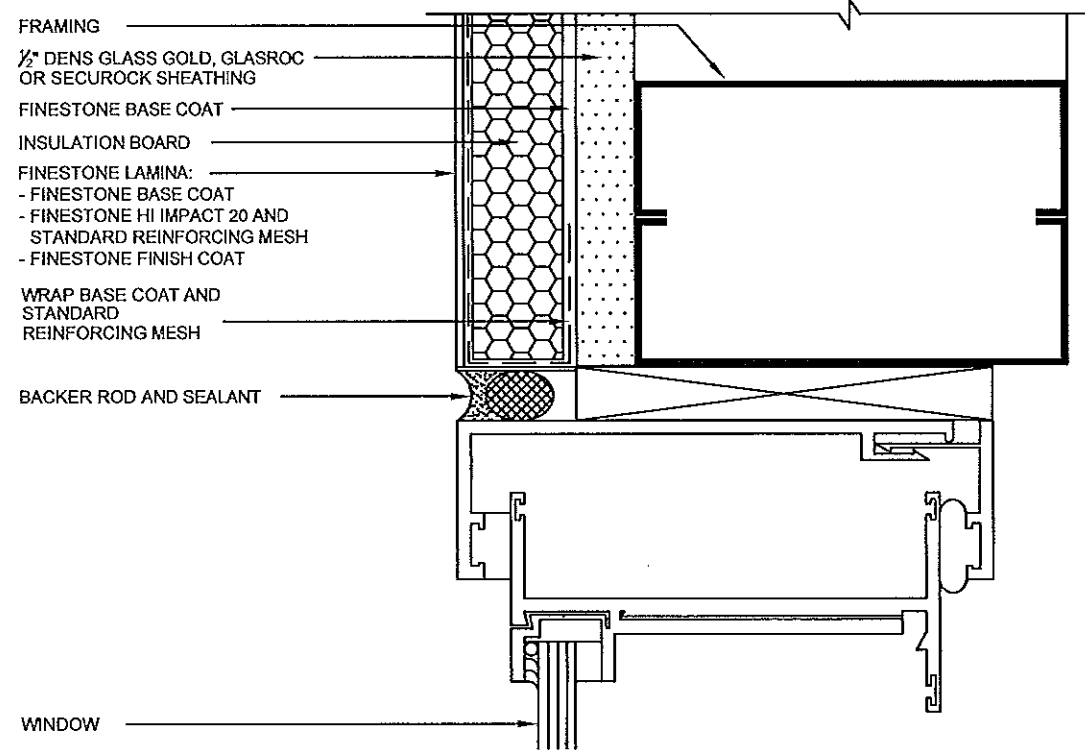
WINDOW JAMB DETAIL (FLUSH)
